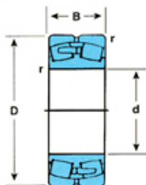
Cylindrical bore 232
